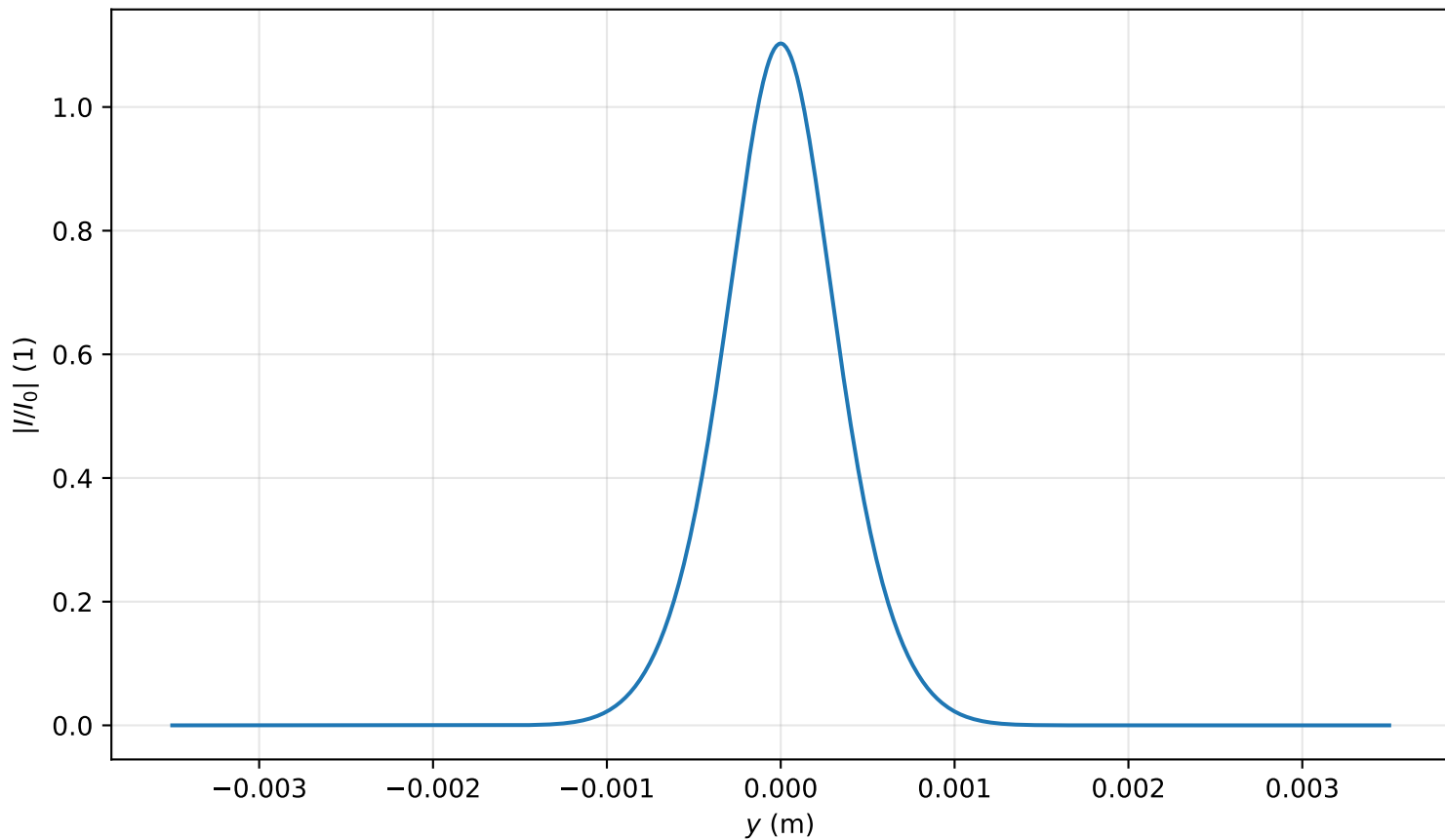
Intensity profile I(x=0, y, z=0.716)/I_0 , P_{in}=0.6P_{cr} , artificial time
